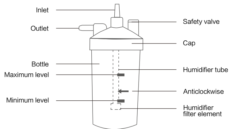
Figure 5: Humidifier Components
