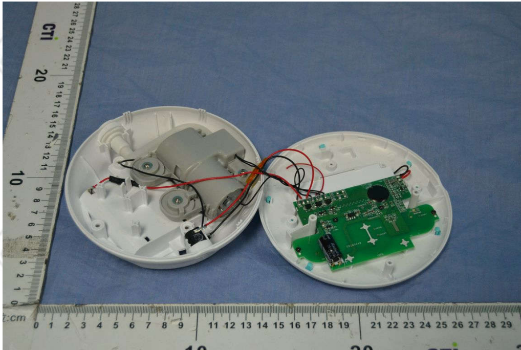
Picture 7 Internal view (Controller)
