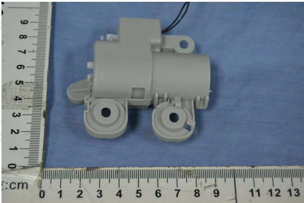
Picture 10 Pump and electromagnetic valve view (With enclosure)
